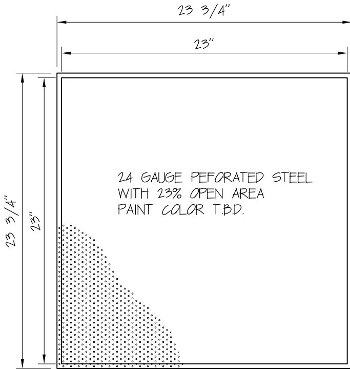
ELEVATION ACOUSTICAL LAY-IN PANEL (ALP)
